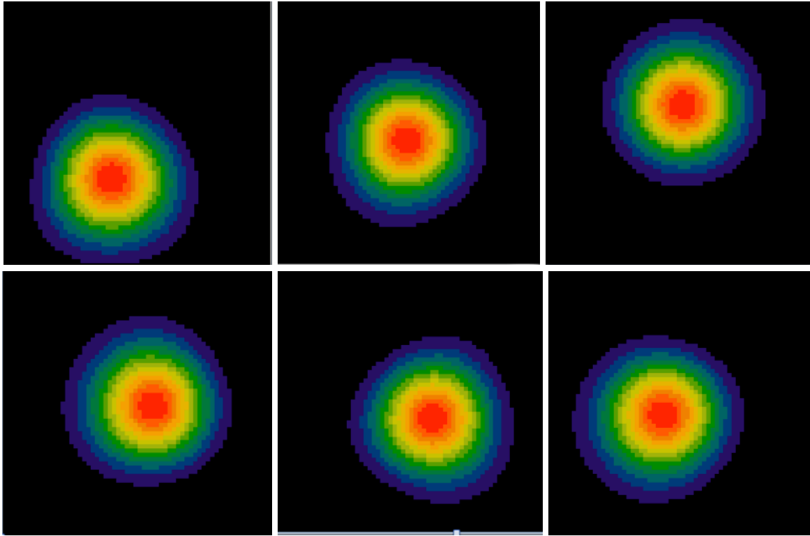
Figure 5. A series of simulated communication beam profile at the LCRD space terminal. The impact of turbulence is mostly seen in the beam wander.
